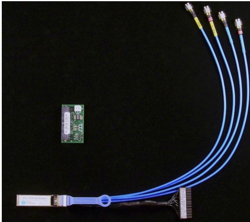
Figure 7. The Wilder SFP+ fixture model number SFP+-TPA-HCB-P, used for SFP+ host electrical testing.
