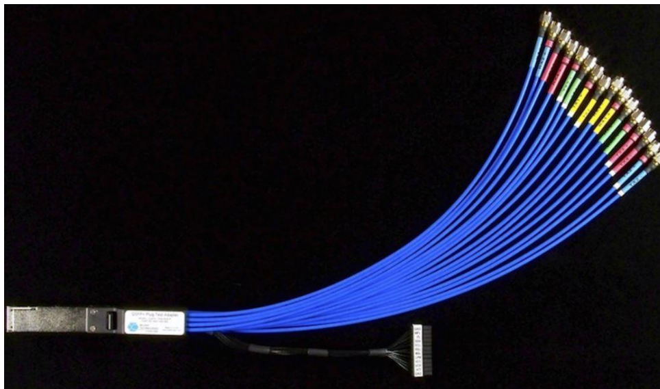
Figure 7. The Wilder SFP+ fixture model number SFP+-TPA-HCB-P, used for SFP+ host electrical testing.
