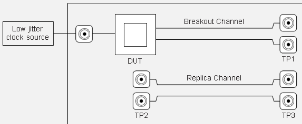
Figure 5: In order to test the transmitter of your PCIe 5.0 silicon, you will need to build or acquire a break-out board that allows you to connect high bandwidth test cables between your ASIC or DUT and your test instrumentation.
