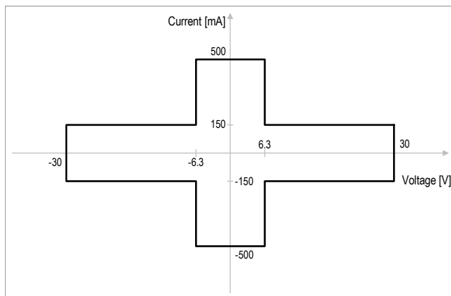
Figure 3. Voltage and current output range per channel
