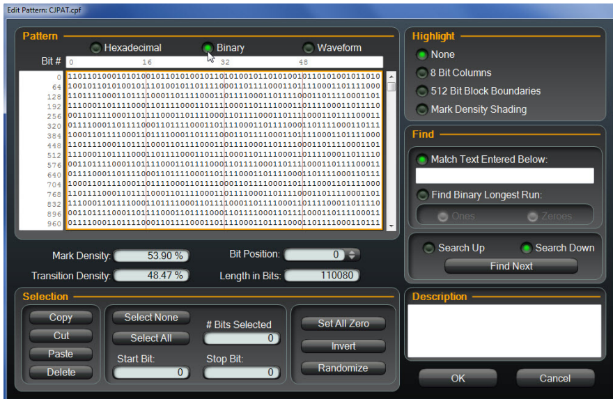
Figure 13. Sub-pattern editor.
