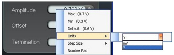
Figure 2. Selecting units.
