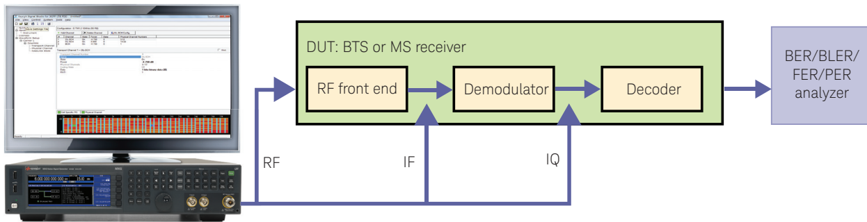
Figure 3. Generate fully channel-coded signals to evaluate the throughput of your receiver with Keysight X-Series signal generators and Signal Studio's advanced capabilities.
