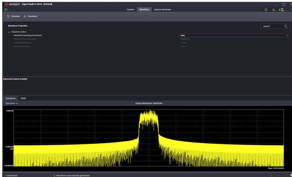
Figure 2. LMR APCO 25 output waveform spectrum view
