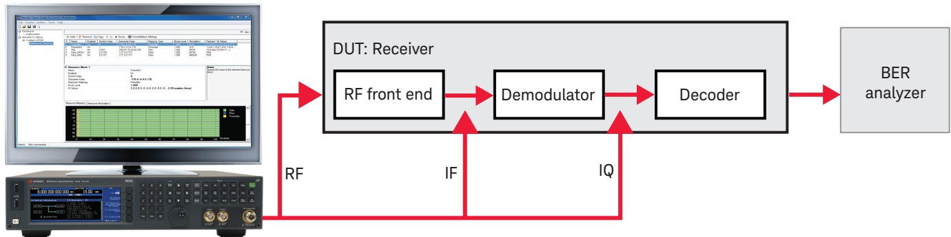
Figure 3. Generate receiver test signals for early testing of your receiver with Keysight X-Series signal generators and Signal Studio.
