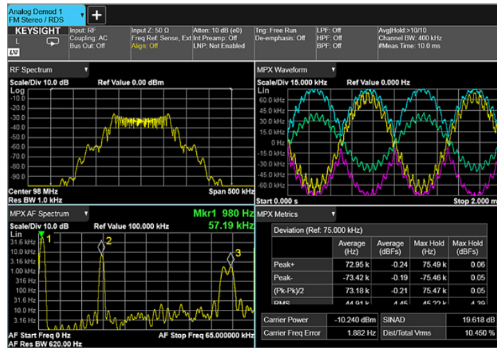
Figure 7. FM stereo MPX view/display with RF spectrum, AF spectrum, demod waveform and demodulation metrics results.
