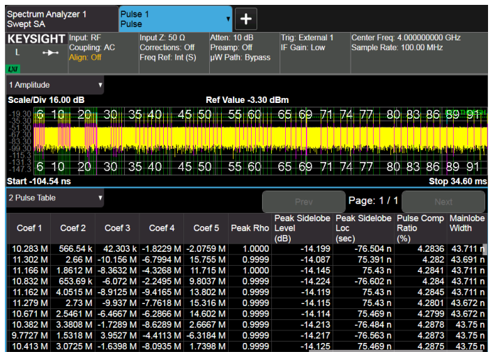
Figure 6. Easily measure pulse linearity and use qualified trigger to select appropriate signal to analyzer.
