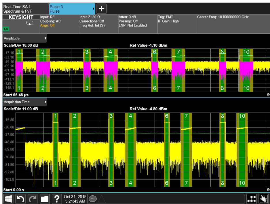
Figure 1. Simultaneous views of pulse signals versus time.
