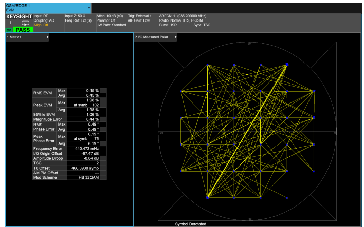
Figure 2. Constellation diagram and error summary of an HSR 32QAM EDGE Evolution signal.
