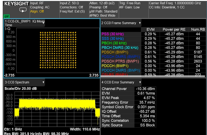
Figure 3. 5G NR Downlink Modulation Analysis measurement
