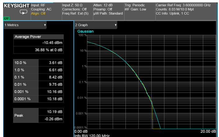
Figure 8. 5G NR CCDF Measurement
