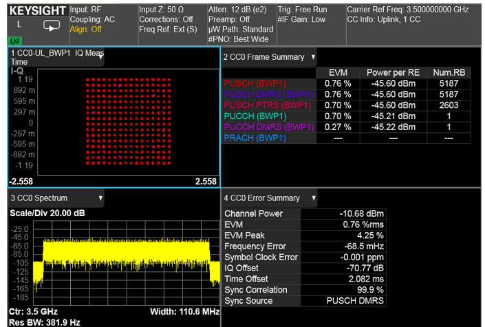
Figure 6. 5G NR Uplink Modulation Analysis measurement
