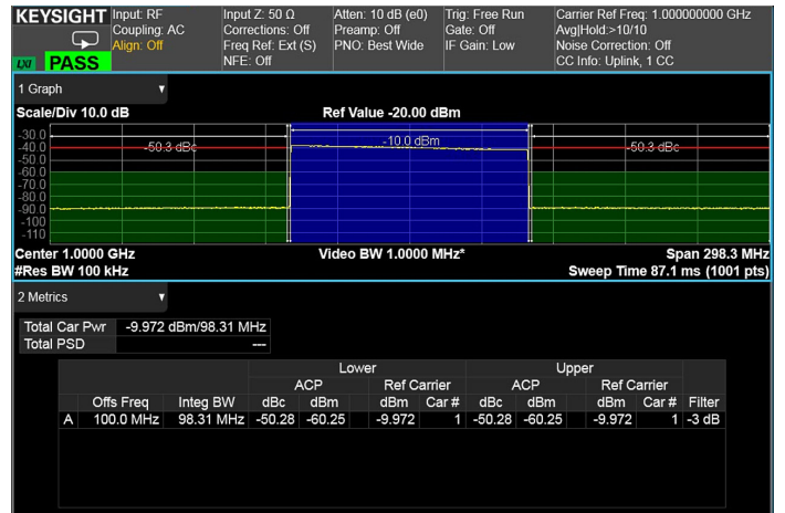
Figure 7. 5G NR ACP Measurement
