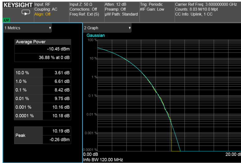
Figure 8. 5G NR CCDF measurement
