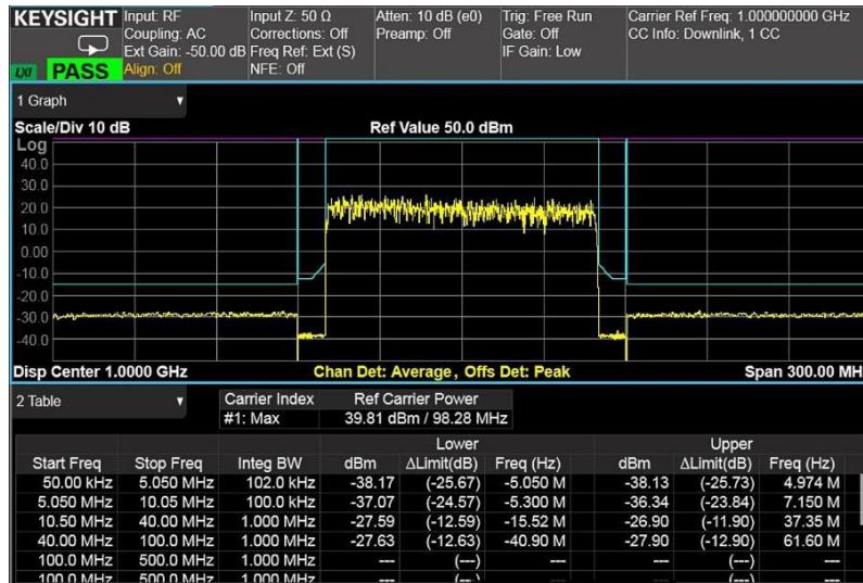
Figure 5. 5G NR Downlink SEM measurement
