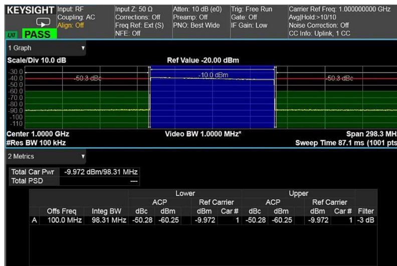
Figure 7. 5G NR ACP measurement
