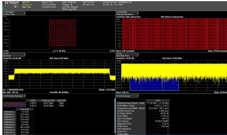
Figure 6. 5G NR Uplink Modulation Analysis measurement
