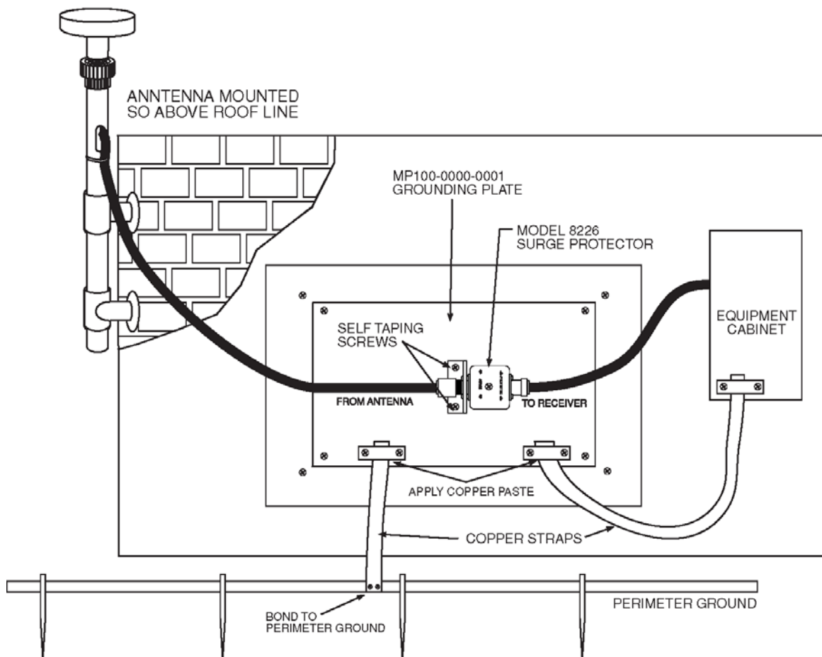
Figure 1-3: Grounding kit panel installation
