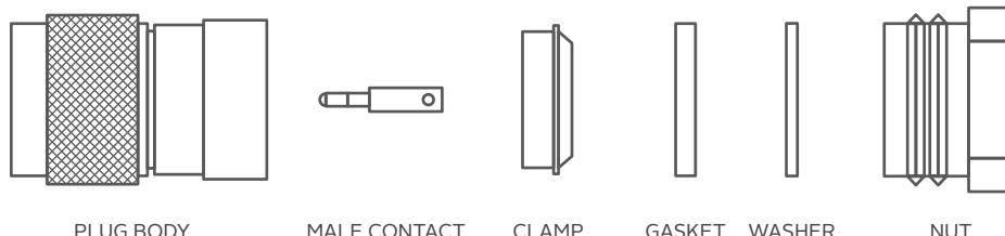
Figure 1-4: Connector component; and below Table 1-1: Connector Assembly
