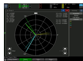
Phasor diagram for phase relationship analysis
