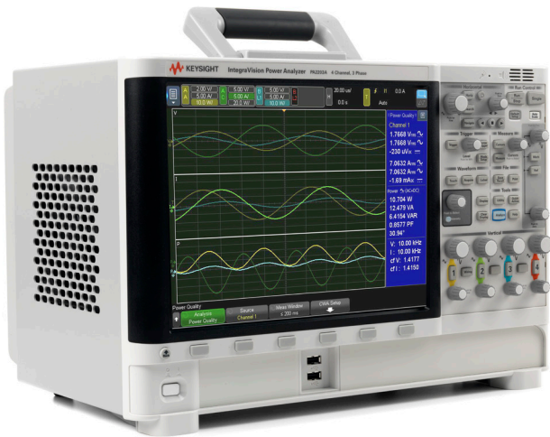
PA2203A IntegraVision Power Analyzer 4 Power Channels, 3-Phase Analysis
