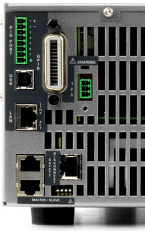
Figure 5. Digital control port on rear panel
