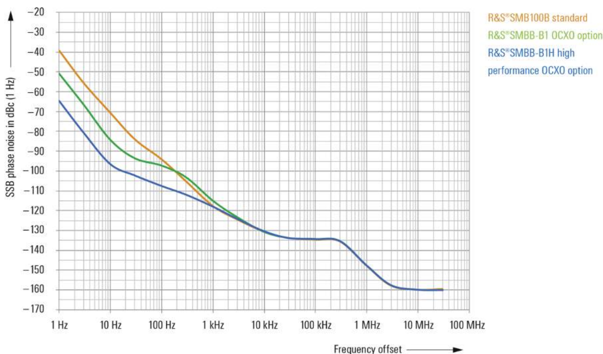
SSB phase noise of the R&S®SMB100B base unit at 1 GHz (measured), with R&S®SMBB-B1 OCXO reference oscillator option and R&S®SMBB-B1H OCXO reference oscillator, high performance option
