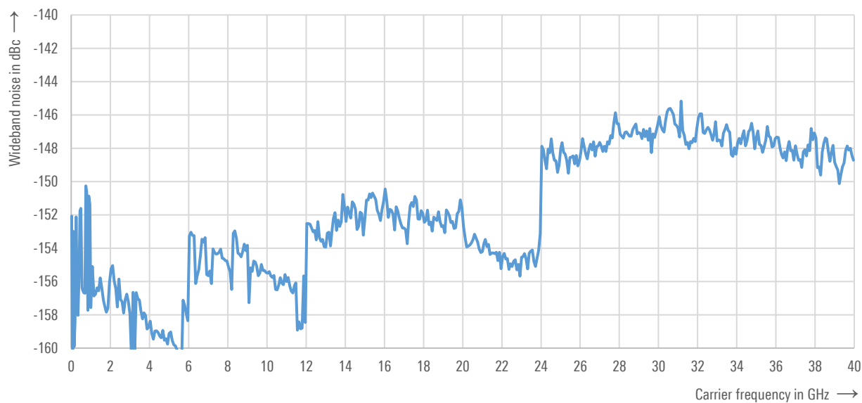
Measured wideband noise (R&S®SMBB-B112/-B120/ B131/-B140(N)), CW, level = +10 dBm
