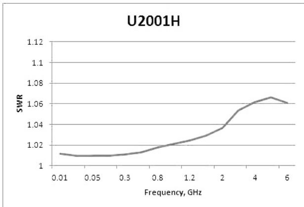
Typical SWR for U2001H sensor (25 °C ± 10 °C)
