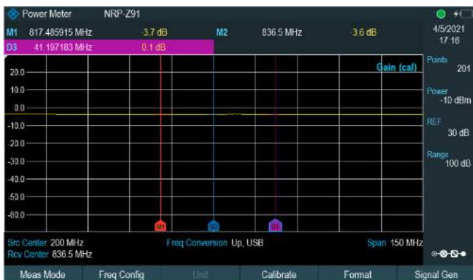
Mixer loss measurement with R&S®ZNH-K69 and the R&S®NRP-Z91 power sensor.
